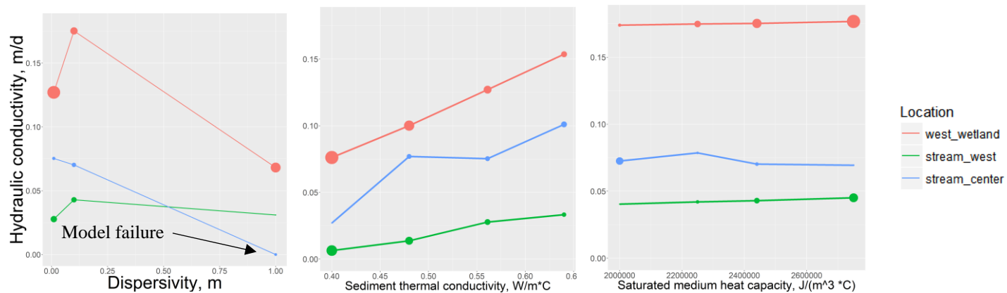
Figure 4: Inverse model sensitivity analysis results. The sensitivity of each hand estimated parameter was tested by running the inverse model over a range of input values and comparing
